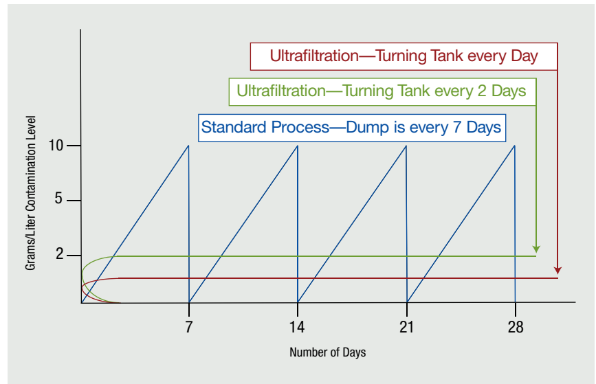
Figure 2: Comparison of contamination levels in a typical aqueous cleaning system and a cleaning system with UF.
